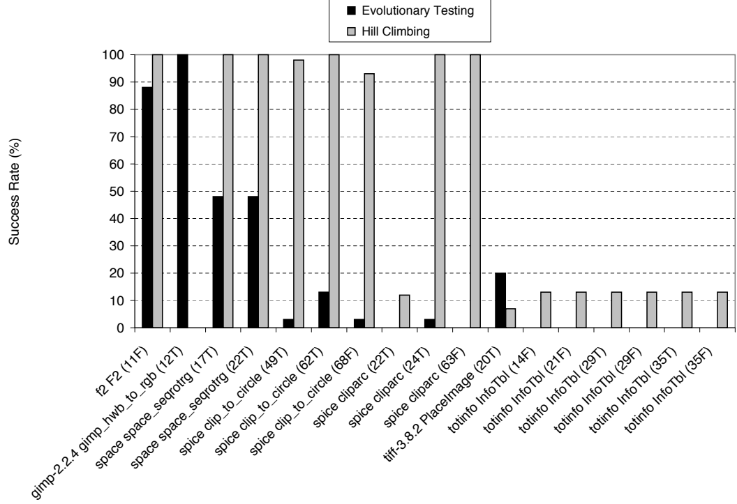
Figure 11: Non Royal Road branches not covered with a 100% success rate by both Evolutionary Testing and Hill Climbing
