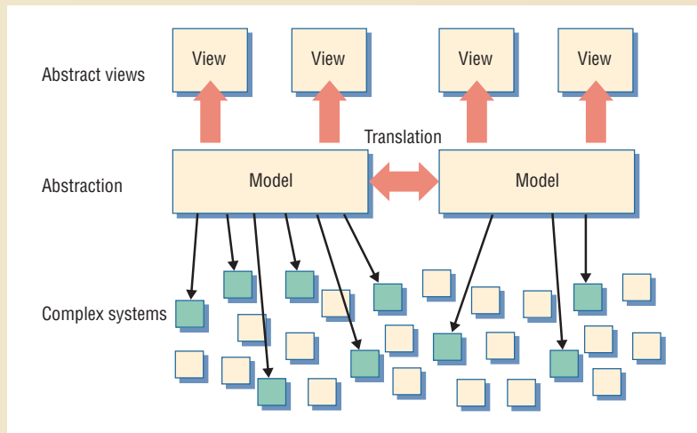
Figure B. Relationship between views, models, and implementation. Rather than replicating the abstractions that programming languages provide, models abstract upon "selected" elements of the implemented complex system.
