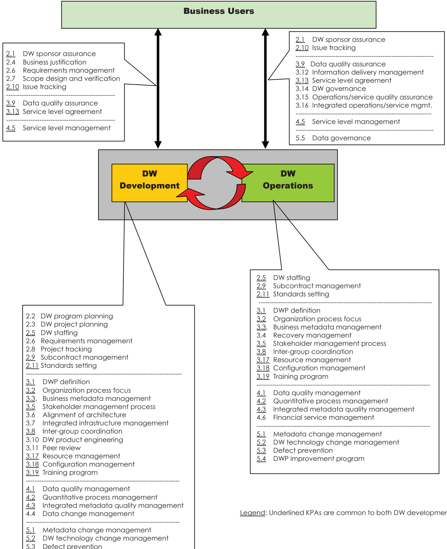
Figure 2. Data Warehousing Process Maturity Model and KPAs (FINAL Version)
