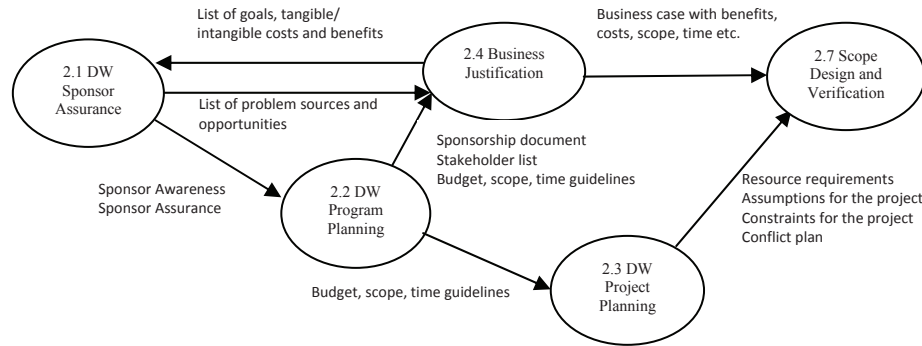
(a) Relationships in Level 2
