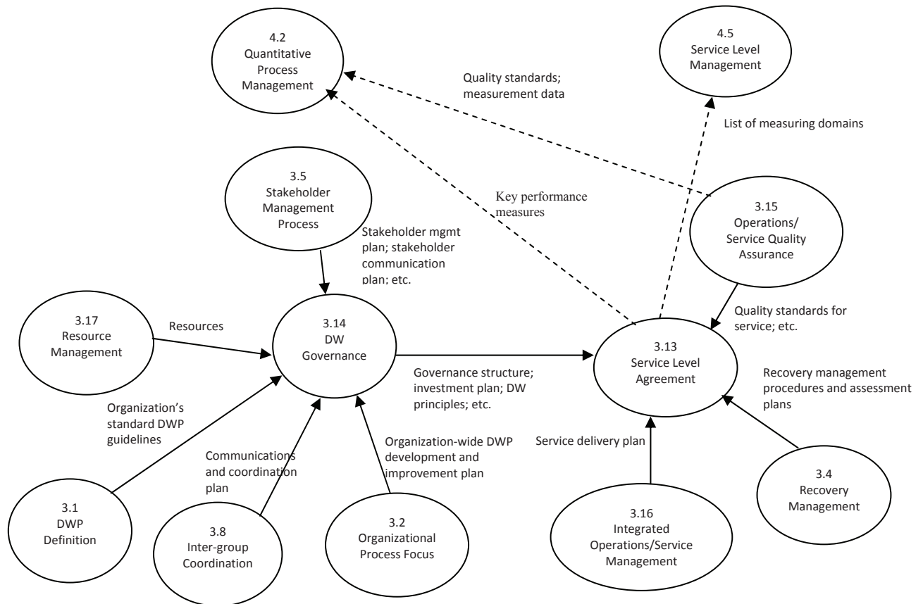
(a) Relationships in Level 2
