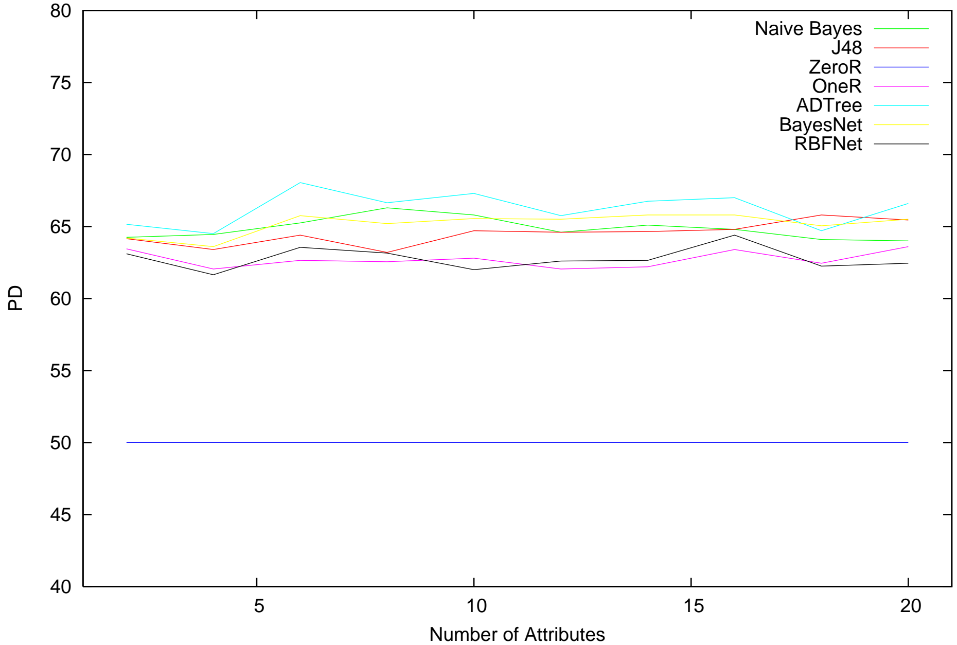
PD - Chi-squared
