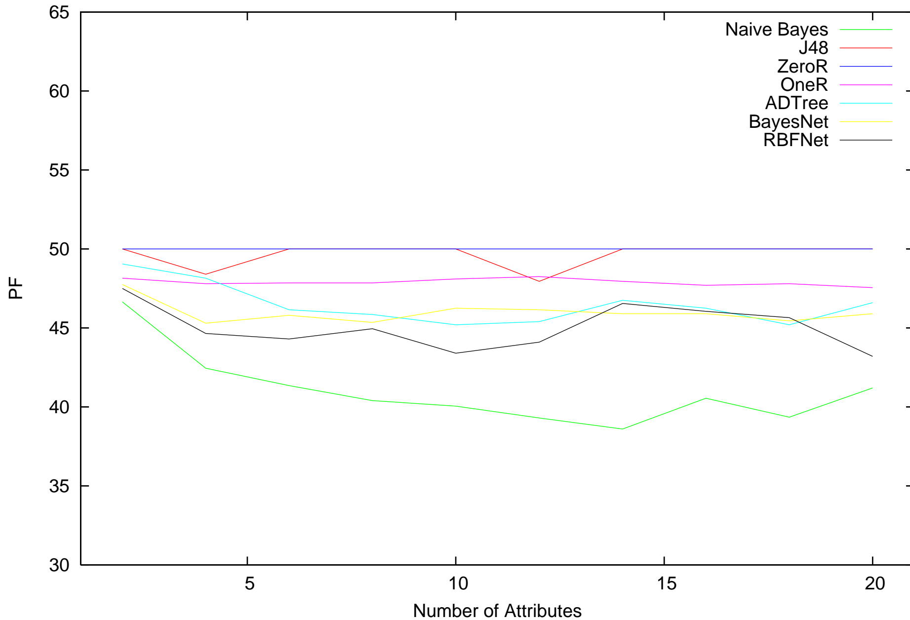
PF - Chi-squared
