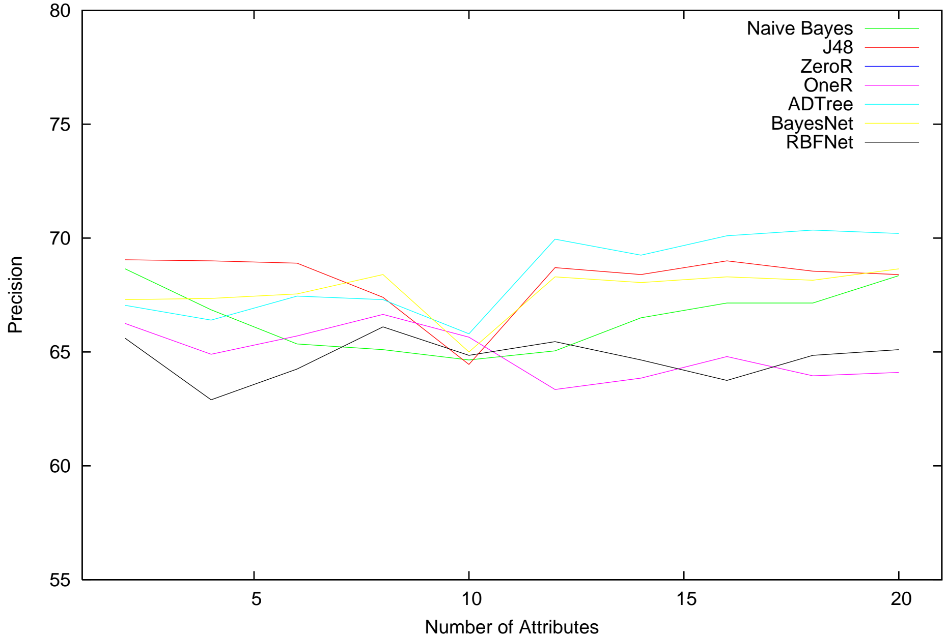
Precision - Chi-squared
