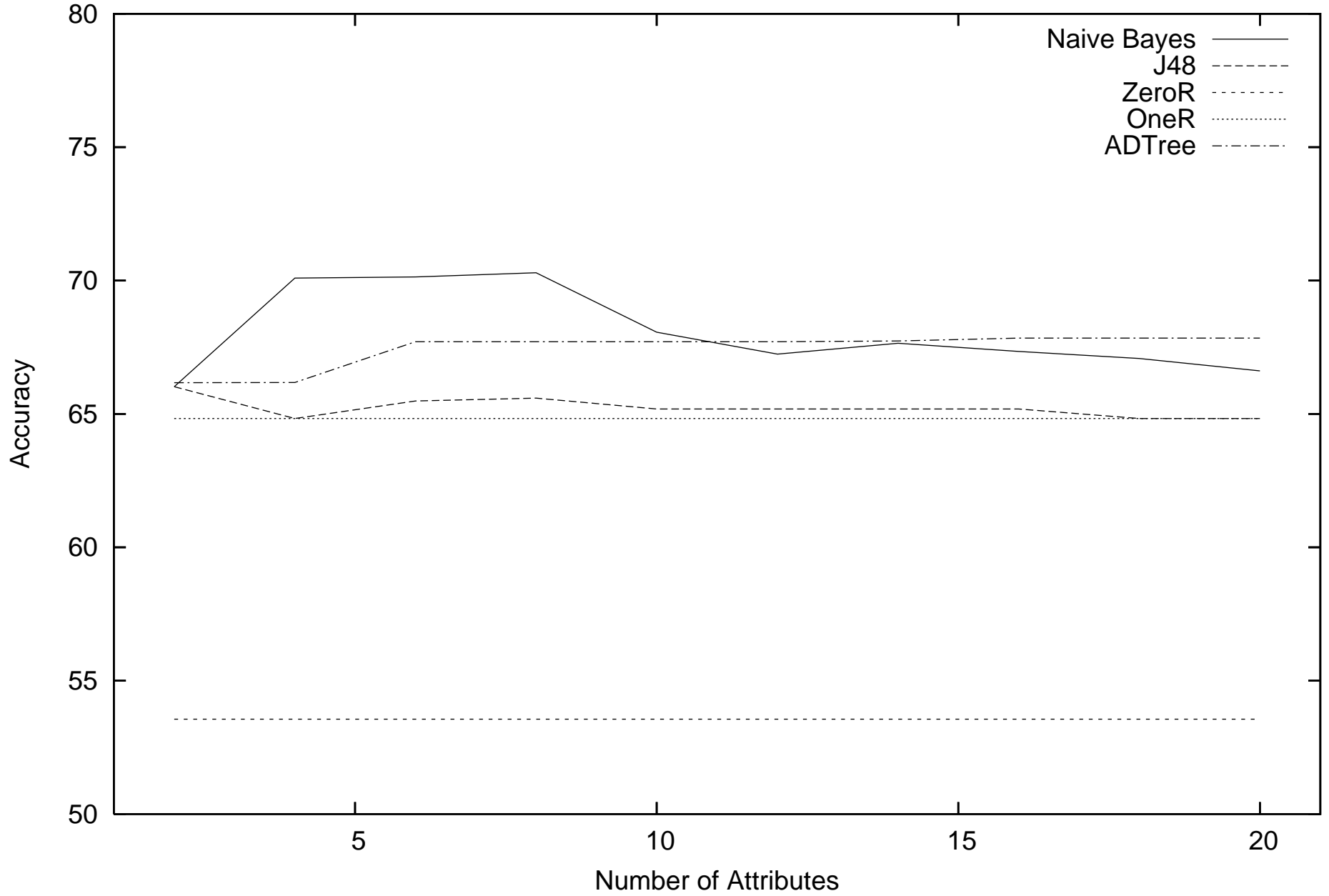
Accuracies
