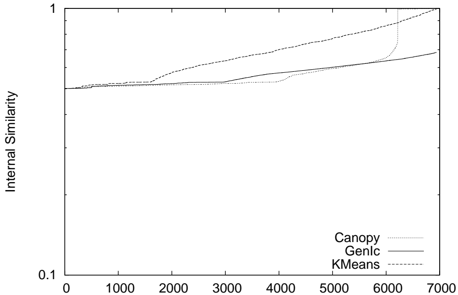
AUC of Internal Similarity by Clustering Method
