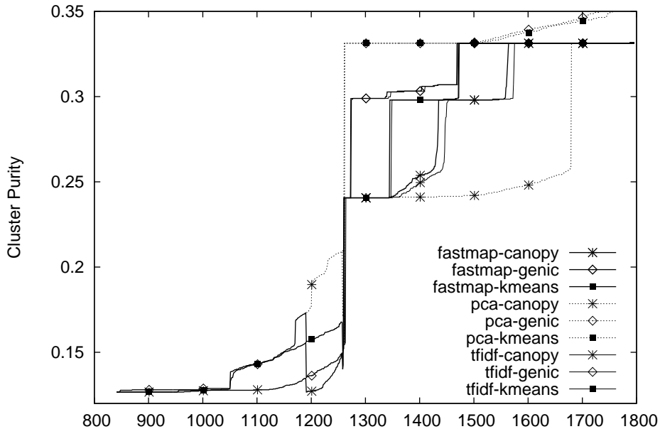
Overall AUC of Cluster Purity
