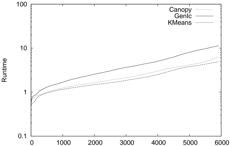
AUC of Runtimes by Clustering Method
