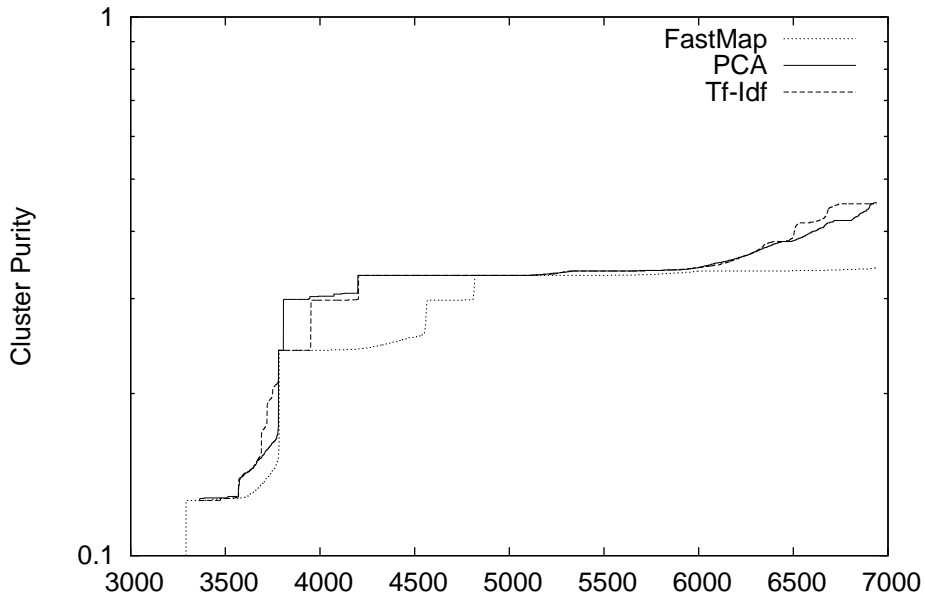
AUC of Cluster Purity by Reduction Method
