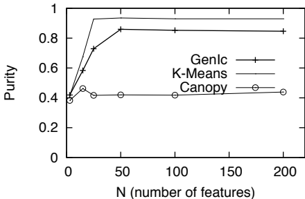
bbcsports - Clustering
