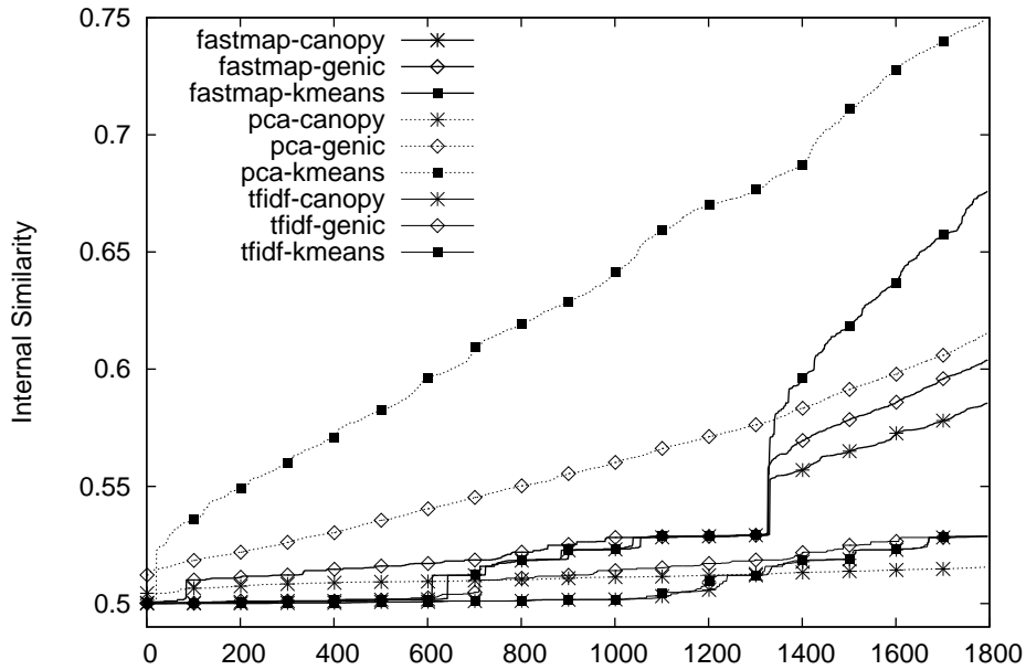
Overall AUC of Internal Similarity
