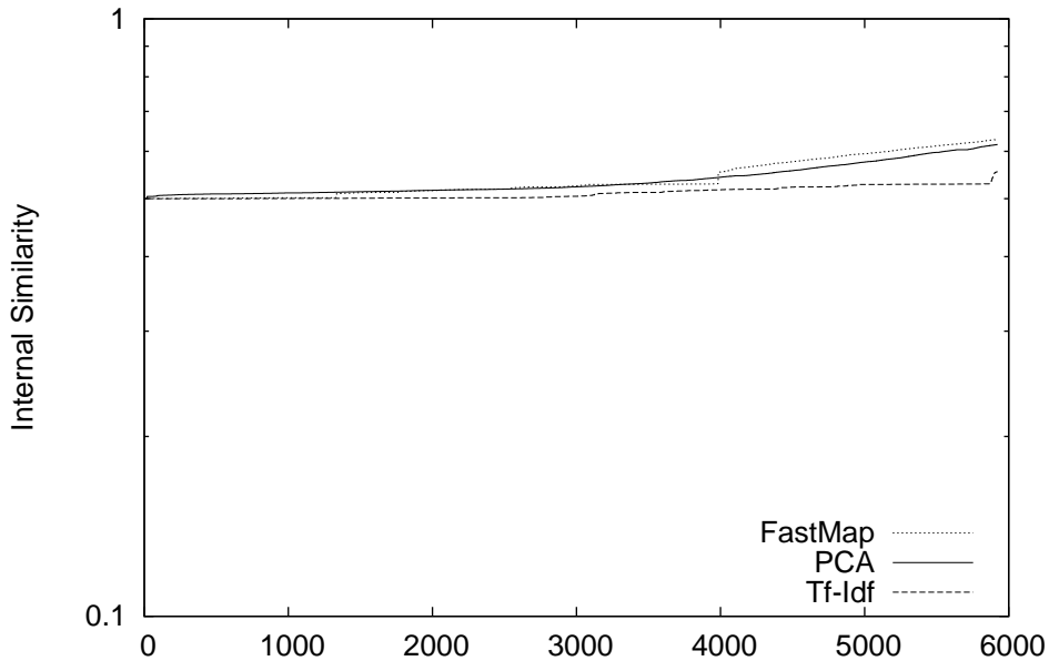
AUC of Internal Similarity by Reduction Method
