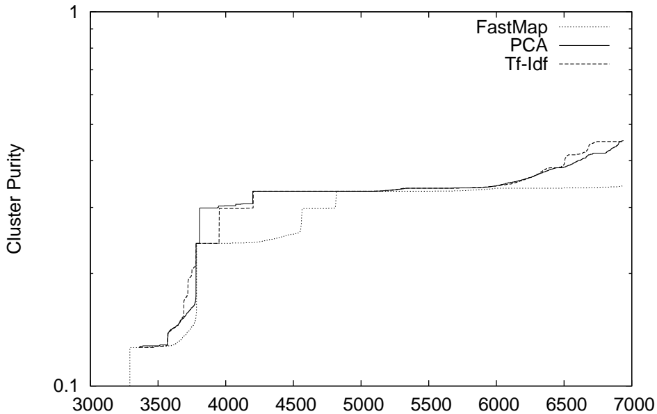
AUC of Cluster Purity by Reduction Method
