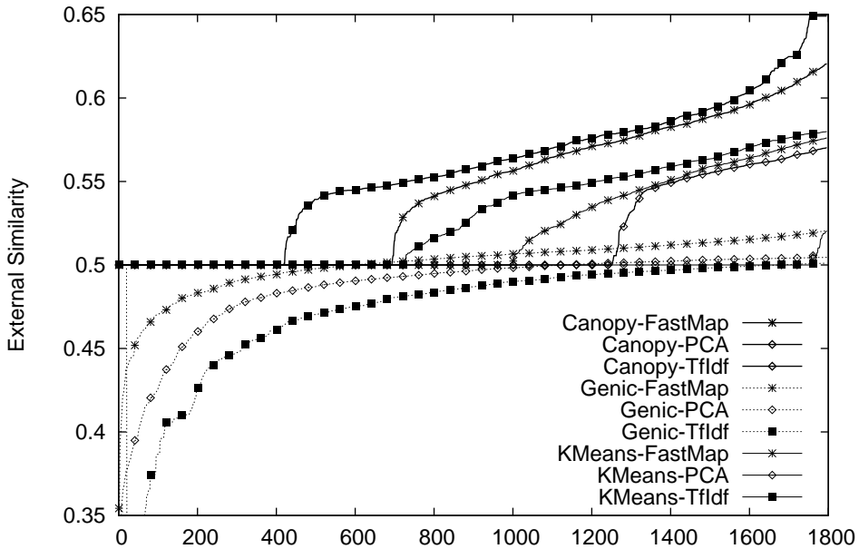
Overall AUC of External Similarity
