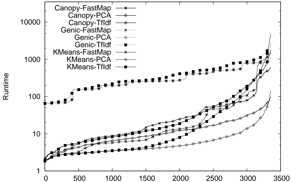
Overall AUC of Runtimes
