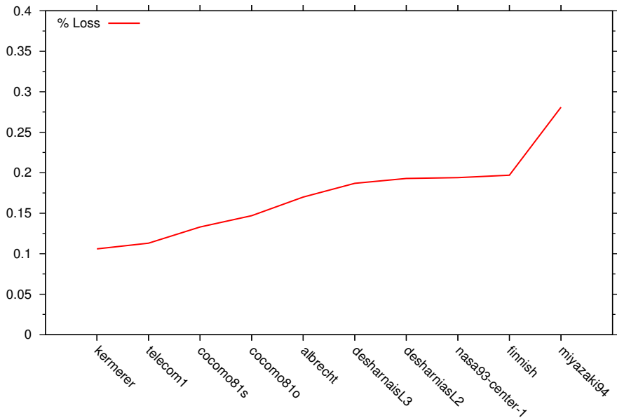
Data Set Win Percentages (pred25)
