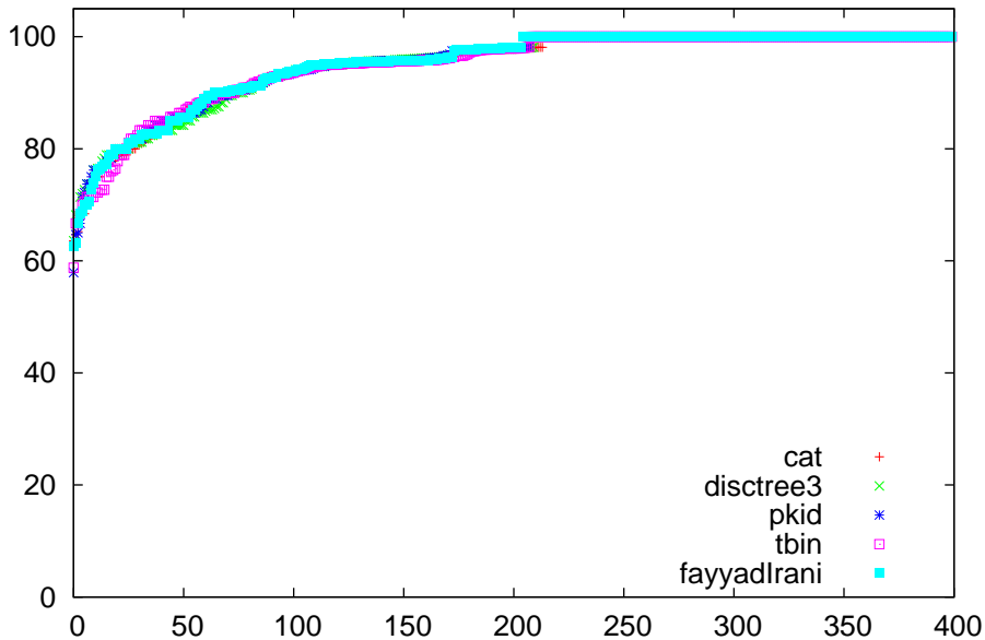
pd comparison for breast-cancer
