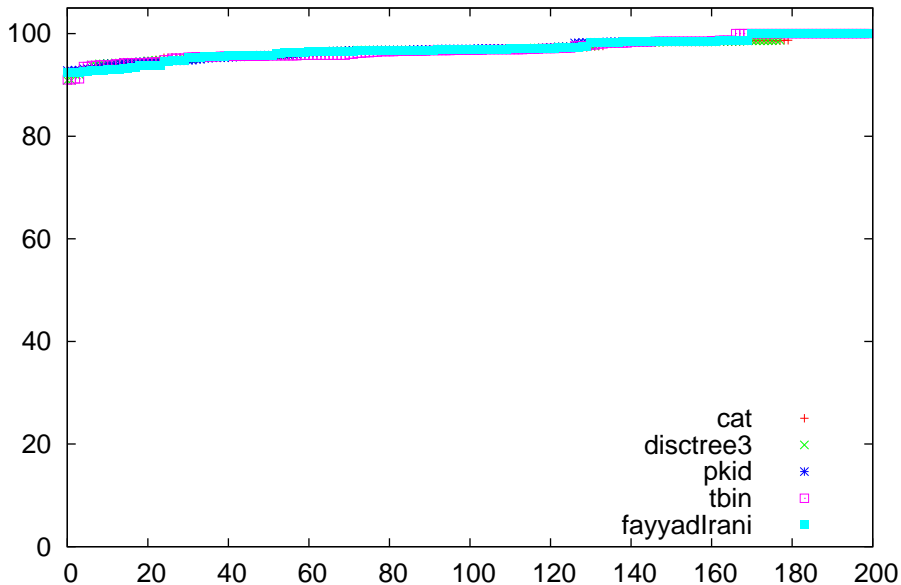
bal comparison for breast-cancer-wisconsin
