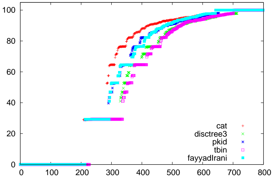
bal comparison for ecoli
