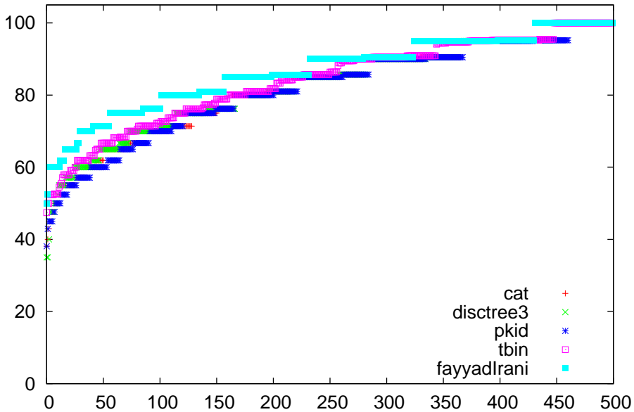
acc comparison for imports-85
