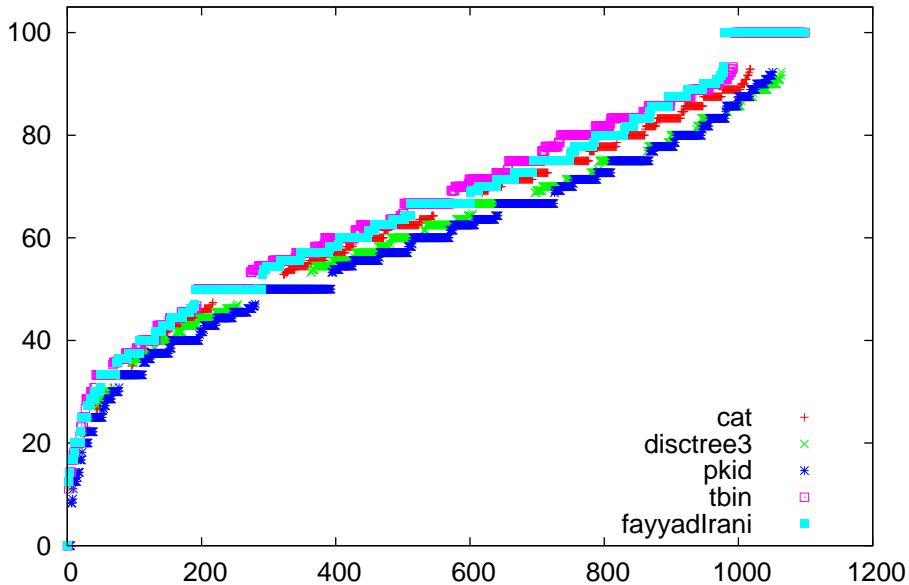
prec comparison for vowel
