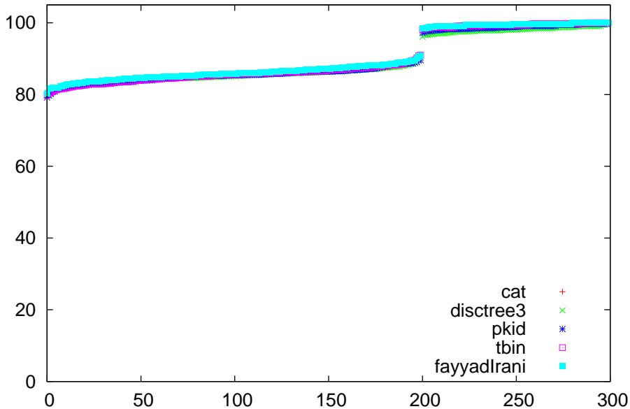
npf comparison for waveform-5000
