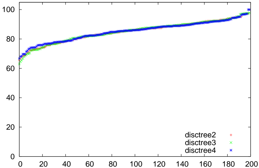
npf comparison for credit-a
