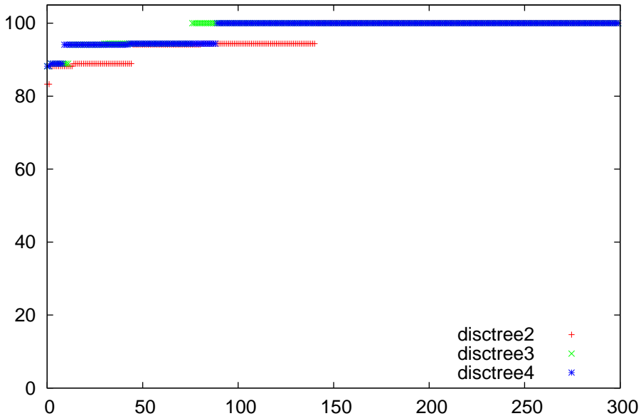
acc comparison for wine
