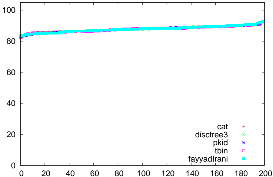
acc comparison for kr-vs-kp
