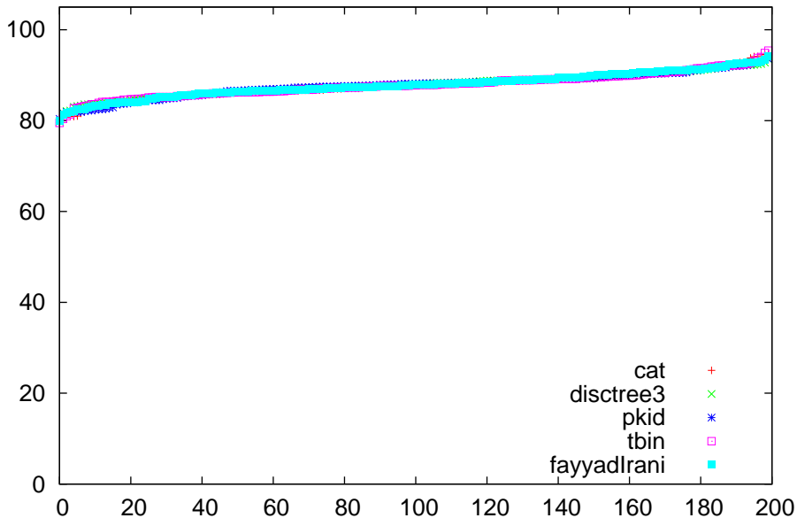
prec comparison for kr-vs-kp
