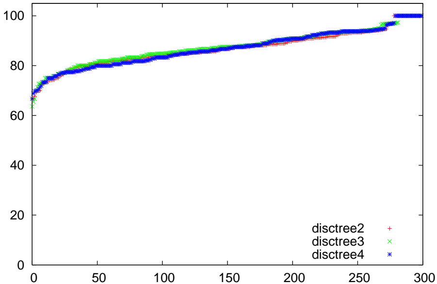
npf comparison for auto-mpg
