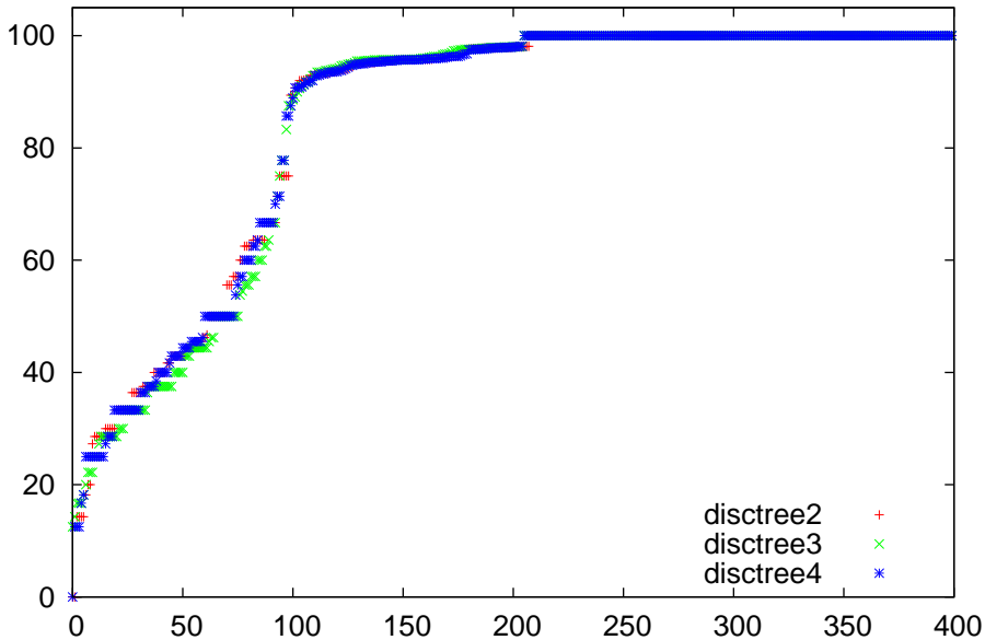
npf comparison for breast-cancer
