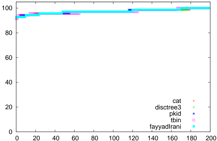
acc comparison for breast-cancer-wisconsin
