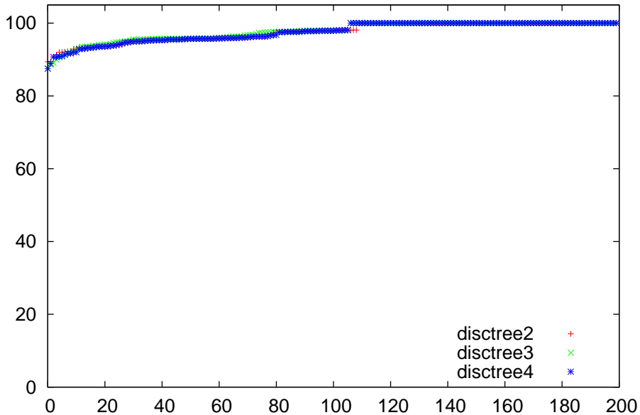
npf comparison for breast-cancer-wisconsin
