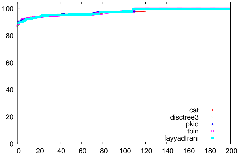
pd comparison for breast-cancer-wisconsin
