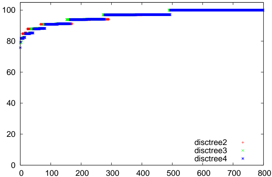
acc comparison for ecoli
