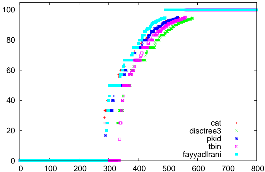
prec comparison for ecoli
