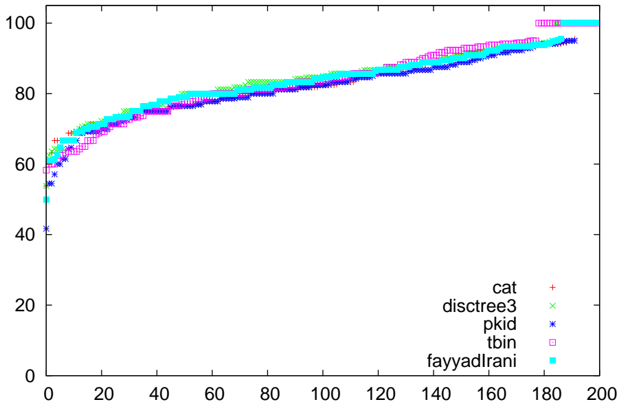
prec comparison for heart-c
