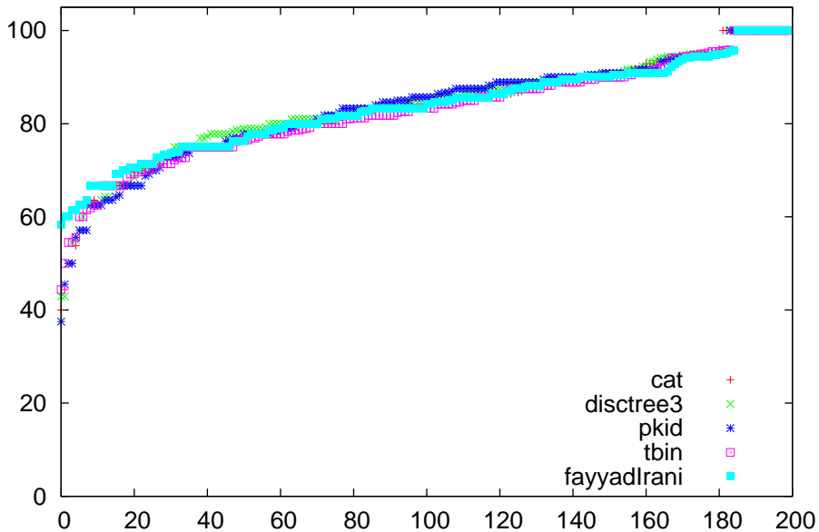
prec comparison for heart-h
