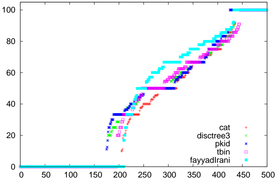
pd comparison for imports-85
