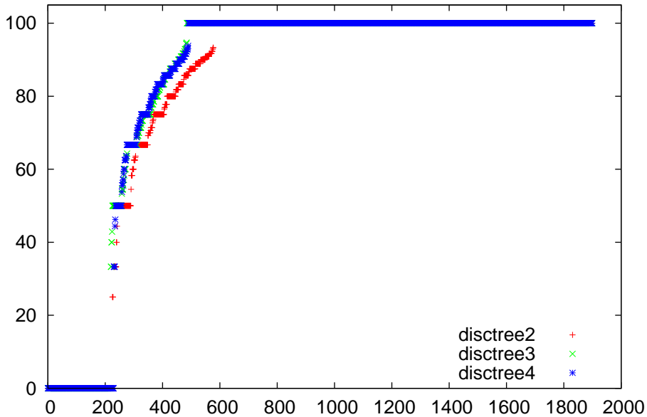
prec comparison for soybean
