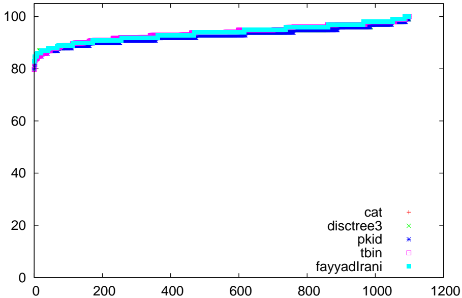
acc comparison for vowel
