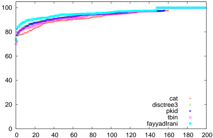
npf comparison for wdbc
