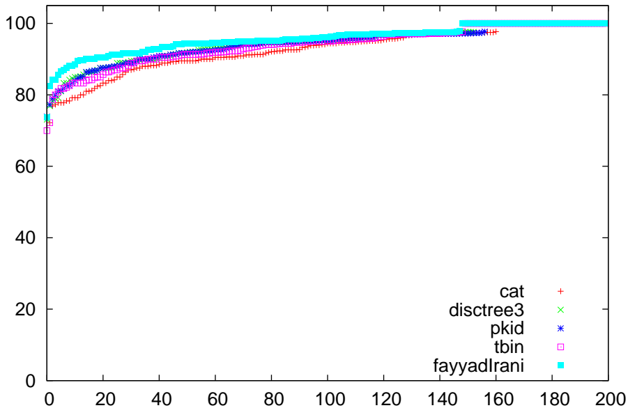
pd comparison for wdbc
