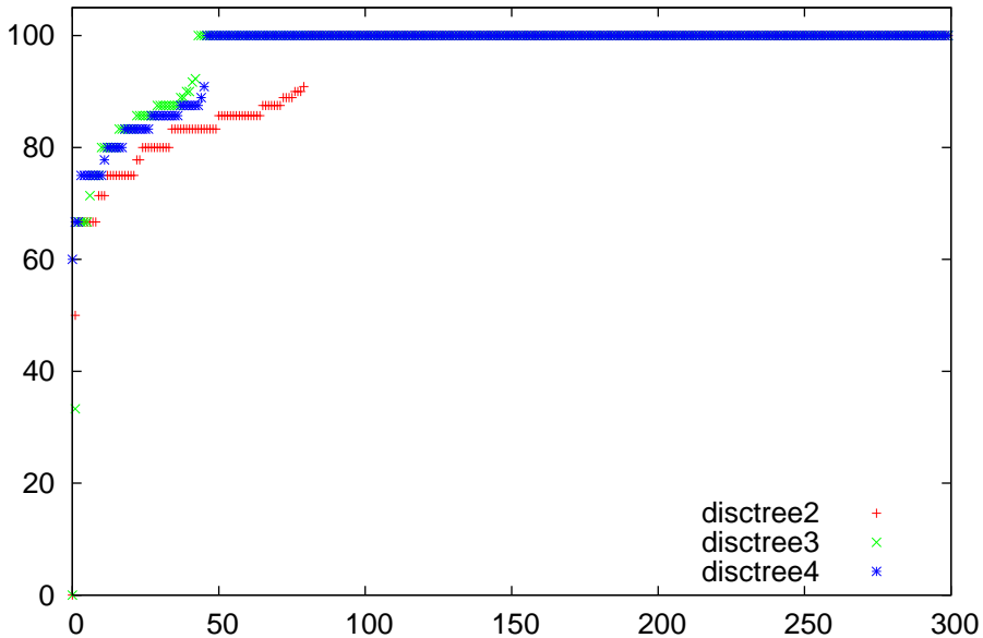
prec comparison for wine
