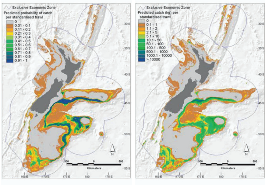
FIGURE 10.21. Geological prediction maps of the presence probability (left map) and catch size (right map) obtained from the gradient boosted models.
