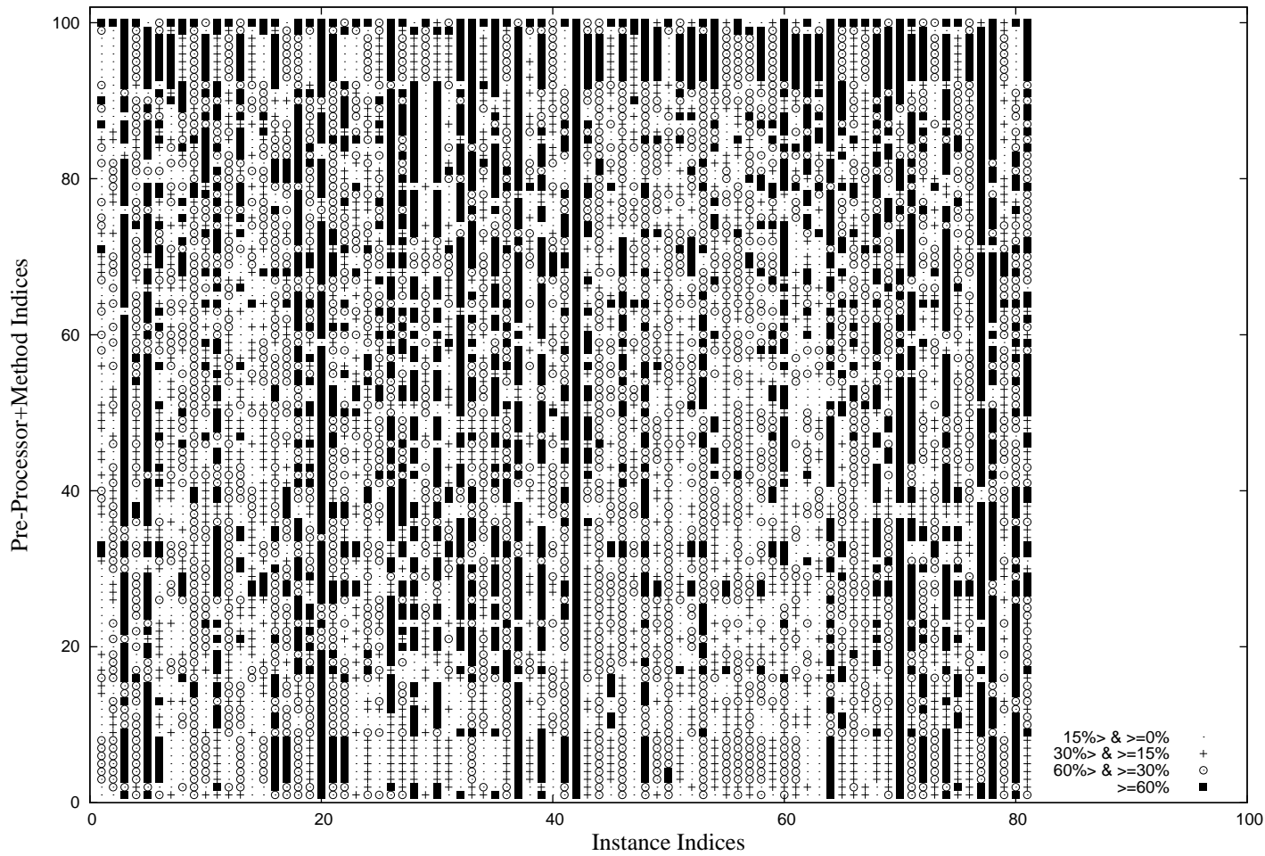
MRE Values for Each Instance In Desharnais Dataset
