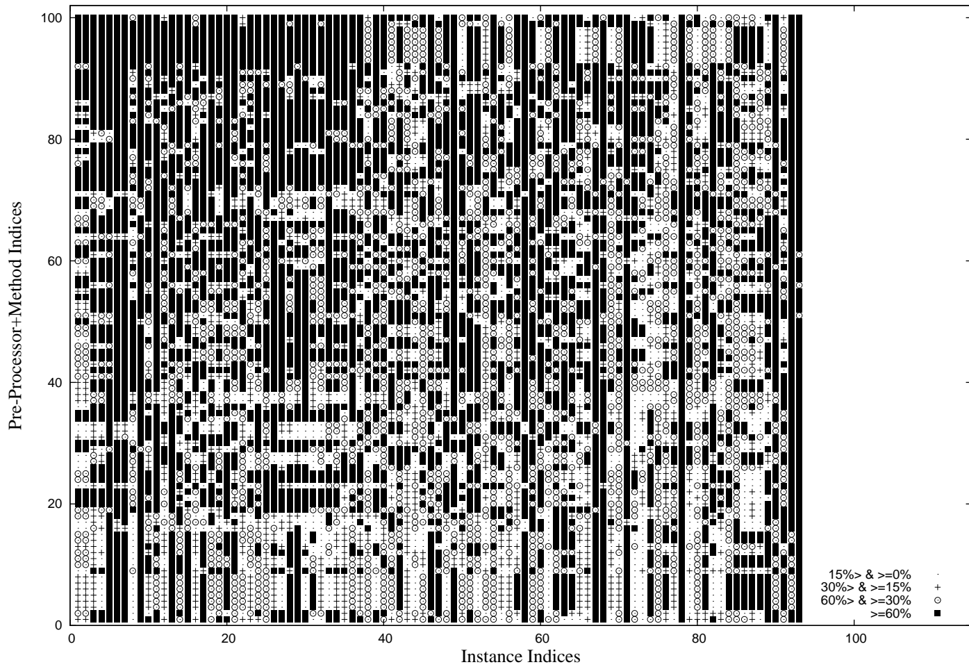
MRE Values for Each Instance In Nasa93 Dataset
