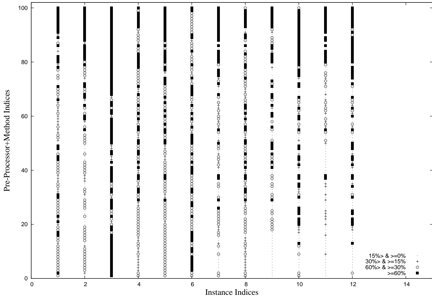
MRE Values for Each Instance In Nasa93c1 Dataset
