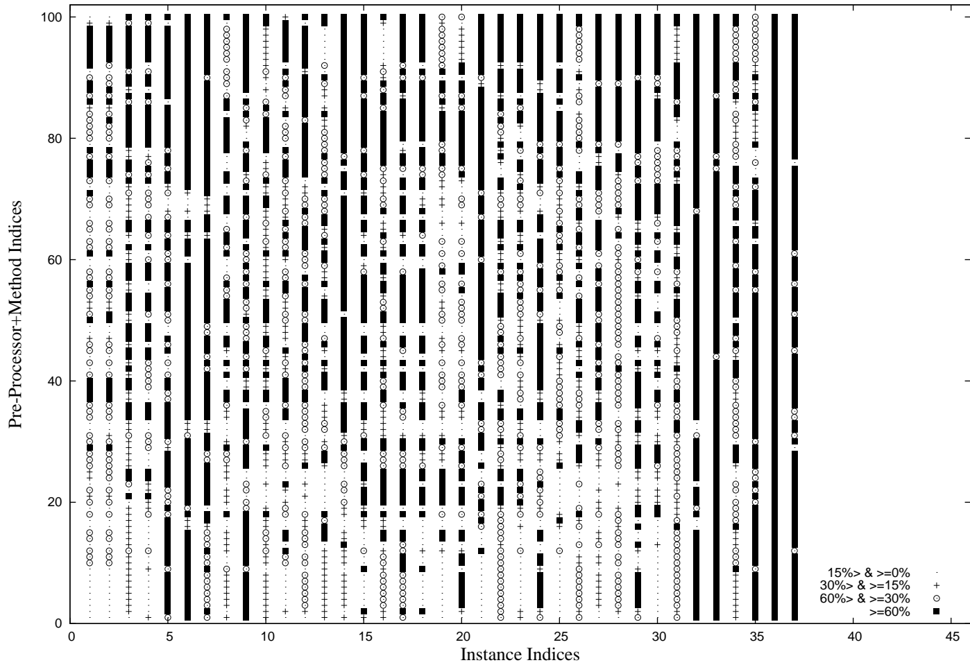
MRE Values for Each Instance In Nasa93c2 Dataset
