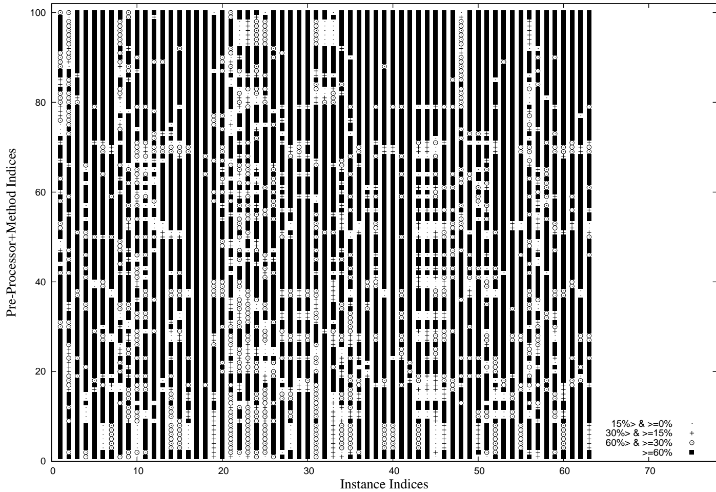
MRE Values for Each Instance In Cocomo81 Dataset
