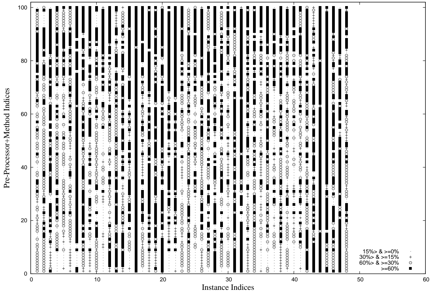
MRE Values for Each Instance In Miyazaki94 Dataset
